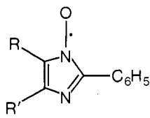
47 122 R = C 6 H 5 SO 2 ; R' = H ( t_{1/2} , CHCl 3 = 2 h) R = C 6 H 5 SO 2 ; R' = C 6 H 5 ( t_{1/2} , CHCl 3 = 10 min) R = R' = CO 2 CH 3 ( t_{1/2} , Et 2 O = 2 h)
