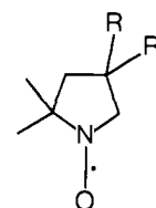
49 123 R = R' = H R = H; R' = CH 3 R = R' = CH 3 ( t_{1/2} , benzene = several hours)
