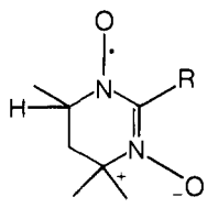
55 128 R = H, Me ( t_{1/2} = "hours")
