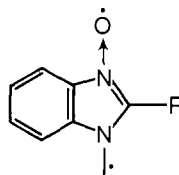
53 R = H 125 R = C 2 H 5 , C 6 H 5 126
