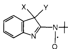
62 135 X, Y = O X = NH 2 ; Y = OH X = CN; Y = OH X = NEt 2 ; Y = OH or NEt 2
