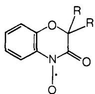
46 , 121 R = H, Me ( t_{1/2} , dioxane = 1 h)
